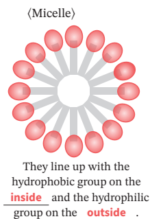
Figure 4-11-2 (Micelle)
